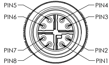
DETAIL A CONNECTOR PIN ASSIGNMENT
